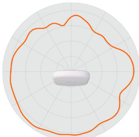
Composite Elevation Outer Trace at 6 GHz
